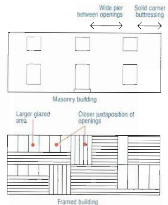
Framed building
